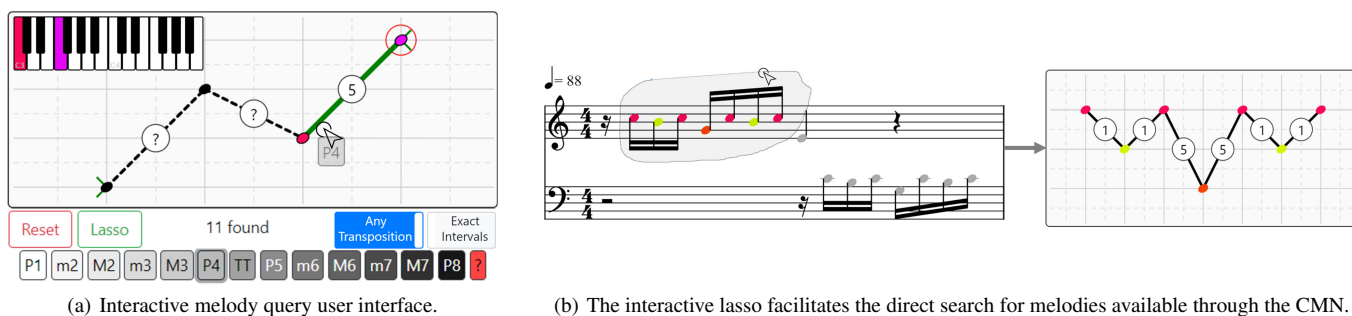
Figure 6: Melody Query. The melody search interface (a) enables analysts to explore melodic patterns. Different parameters allow to create custom queries by assigning intervals or pitches. The lasso selector (b) allows for querying existing melody themes directly from the CMN.
